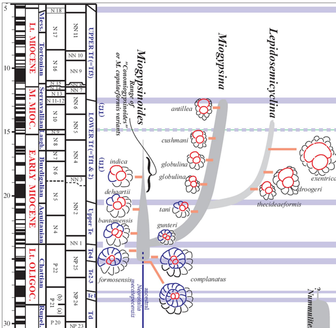
Figure 9. Schematic view of Late Oligocene- Middle Miocene evolutionary development of miogypsinid embryonic stages, mainly based on work of Tan Sin Hok (from Lunt and Allan 2004).
