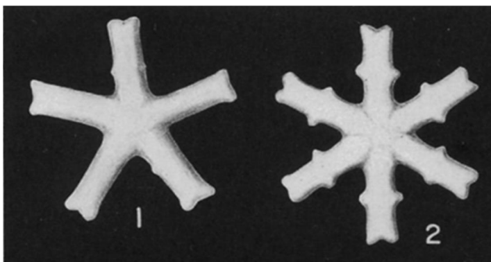
Figure 6. Discoaster tani and Discoaster tani nodifer ; a new species and subspecies named after Tan Sin Hok by Bramlette and Riedel (1954).
